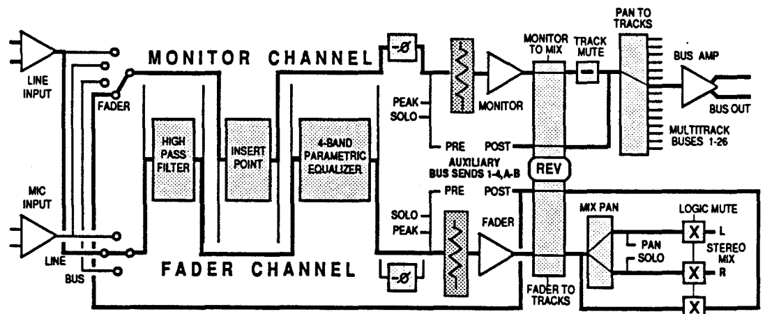
Signal flow in the Elite input module, using REV and the Monitor fader as an echo send master when mixing; the Monitor channel has a processor inserted and is polarity inverted, the Fader channel uses the high pass filter and EQ
